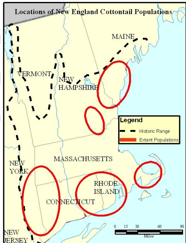
Figure 1. Distribution of Five Extant NEC Populations within the Species' Historical Range (adapted from Nelson 1909; Litvaitis and Litvaitis 1996, p. 725).
